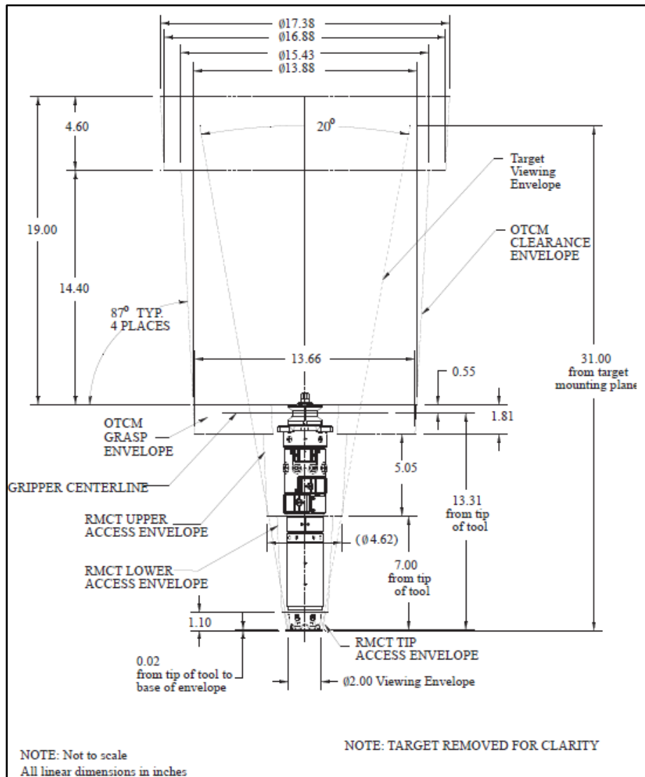
FIGURE 3.1.1-5 RMCT CLEARANCE ENVELOPE
