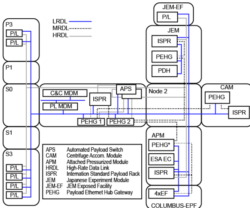
FIGURE 3.0-3 ISS C&DH ARCHITECTURE DIAGRAM
