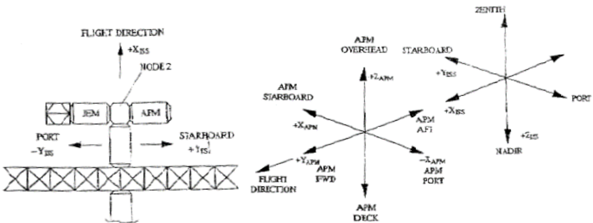
FIGURE 4.3-3 APM/ISS REFERENCE COORDINATE SYSTEM
