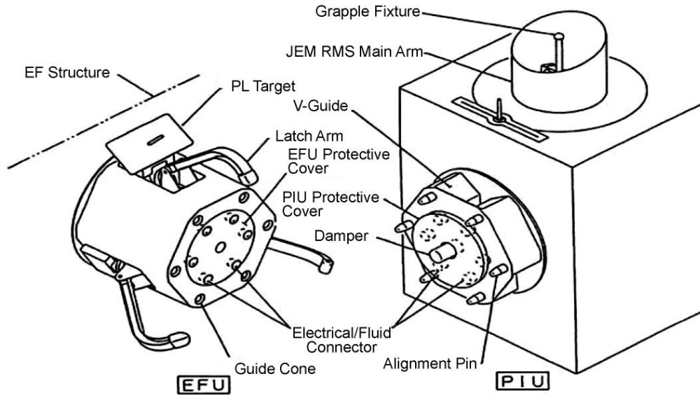
FIGURE 4.2.1-3 PAYLOAD INTERFACE UNIT
