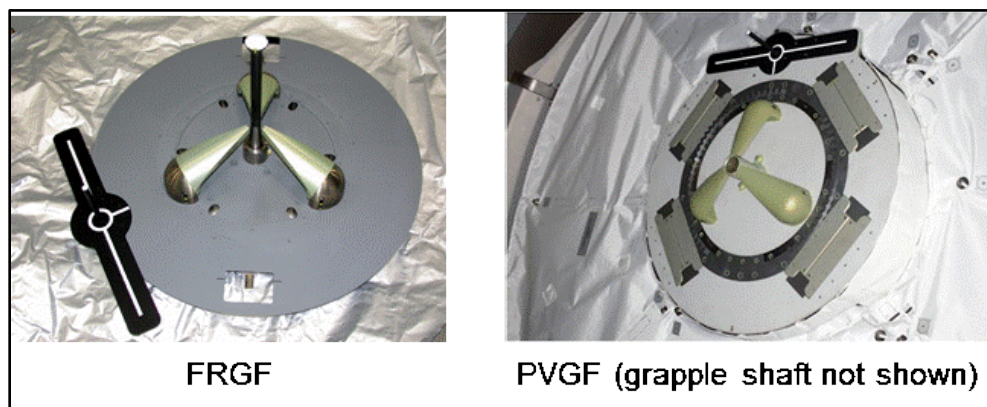
FIGURE 3.1.1-7 SSRMS GRAPPLE FIXTURES
