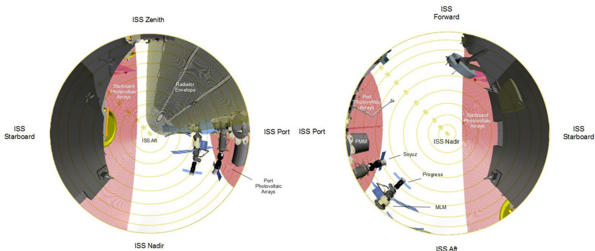
FIGURE 4.1.8-8 ELC-4 INBOARD EXPA PAYLOAD ACCOMMODATION AFT (WAKE) AND NADIR FOVS
