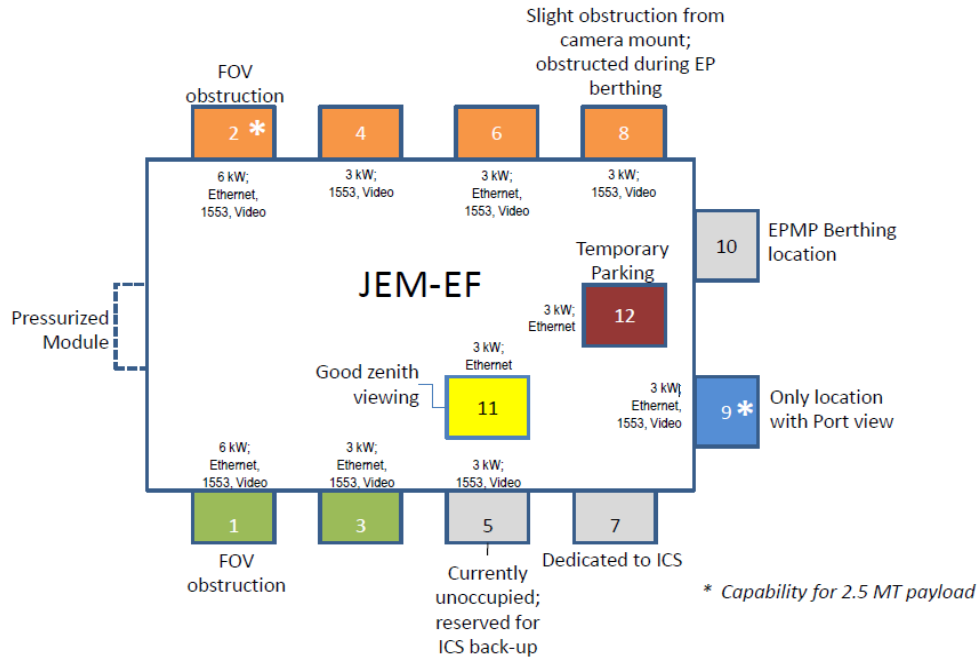
FIGURE 4.2.1-1 ILLUSTRATED JEM-EF 10 LOCATIONS FOR EXPERIMENTAL PAYLOADS
