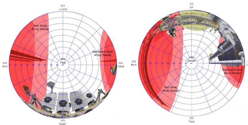
FIGURE 4.2.7-17 JEM-EF EFU11 PAYLOAD ACCOMMODATION FORWARD (RAM) AND ZENITH
