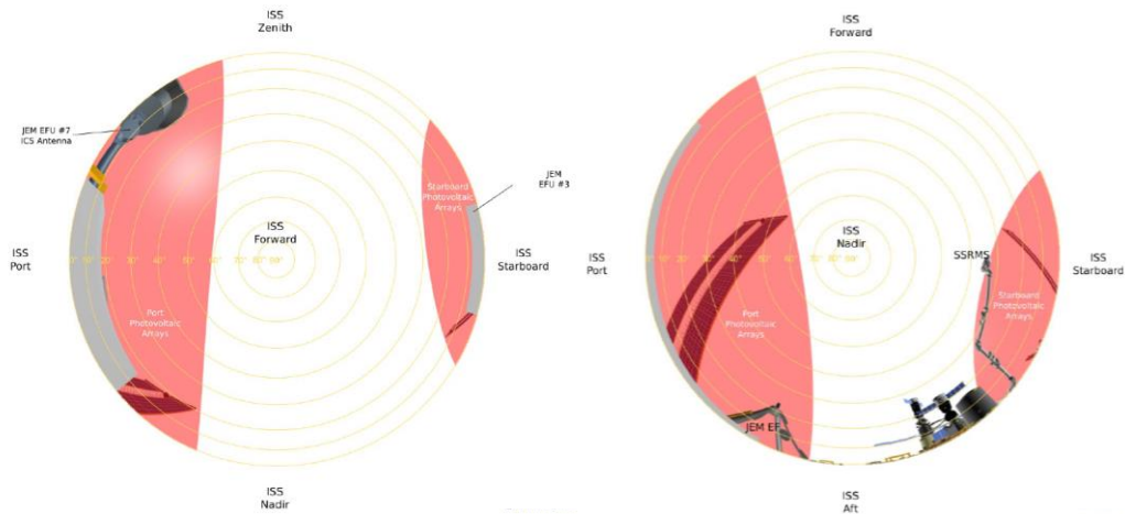
FIGURE 4.2.7-10 JEM-EF EFU5 PAYLOAD ACCOMMODATION FORWARD (RAM) AND NADIR)
