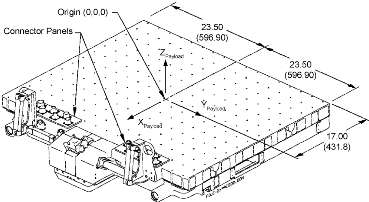
FIGURE 4.1.2-4 GENERIC EXPA PAYLOAD COORDINATE SYSTEM
