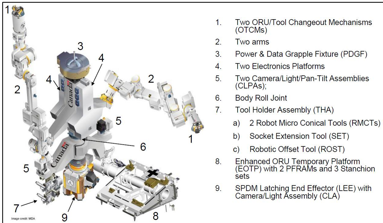
FIGURE 3.1.1-1 ISS DEXTRE
