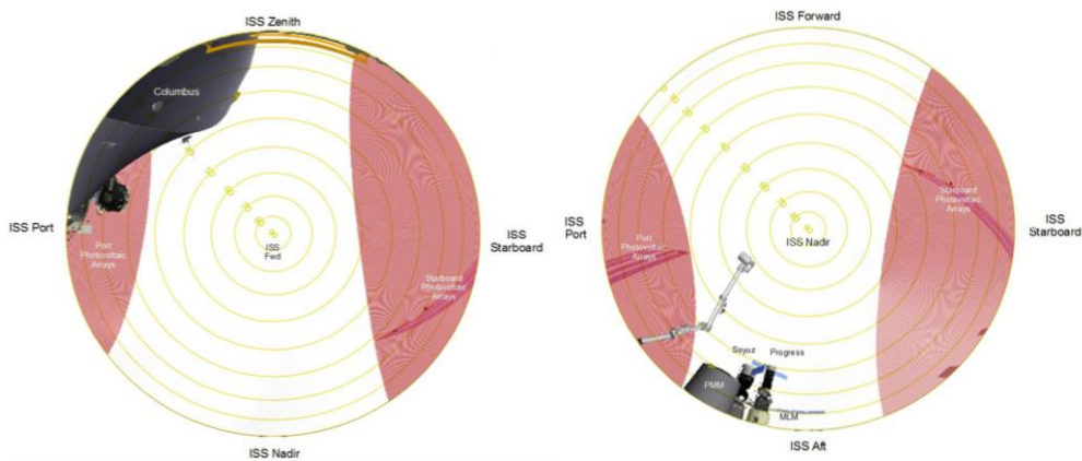
FIGURE 4.3.7-3 COLUMBUS SDN EXPA PAYLOAD ACCOMMODATION FORWARD (RAM) AND NADIR
