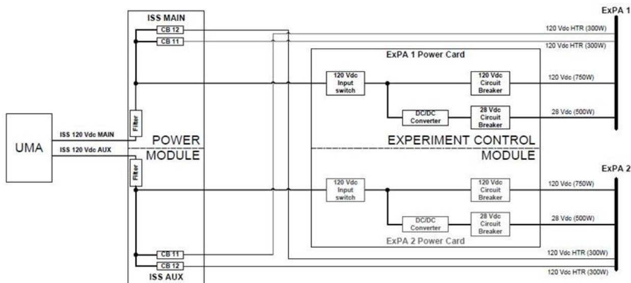
FIGURE 4.1.5-2 ISS TO EXPA POWER BLOCK DIAGRAM
