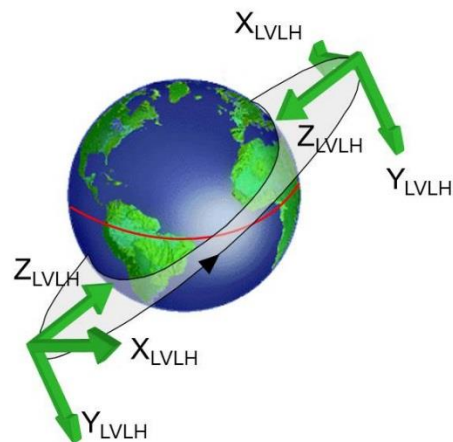
FIGURE 3.1.5-2 LVLH REFERENCE
