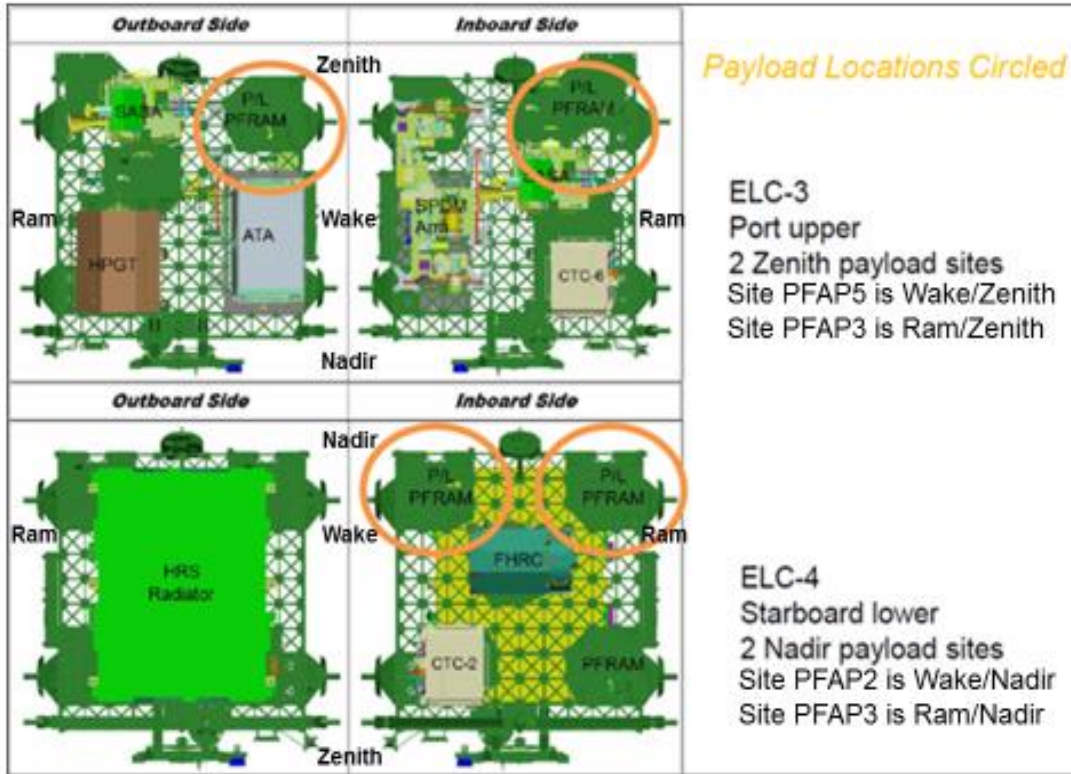
FIGURE 4.1.2-2 ELC LOCATION ON ISS
