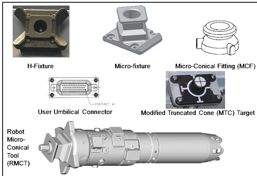
FIGURE 3.1.1-3 DEXTRE INTERFACES
