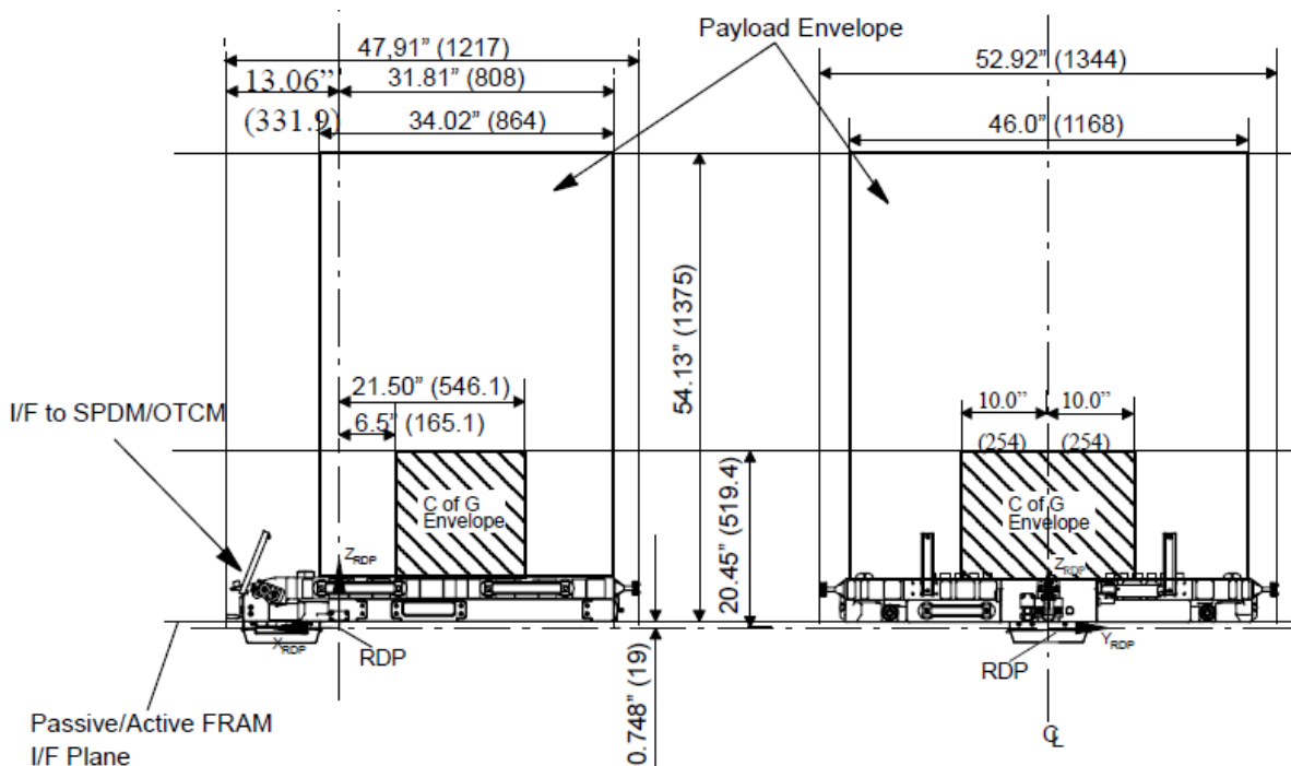
FIGURE 4.3.1-3 INTEGRATED EXTERNAL PAYLOAD ENVELOPE
