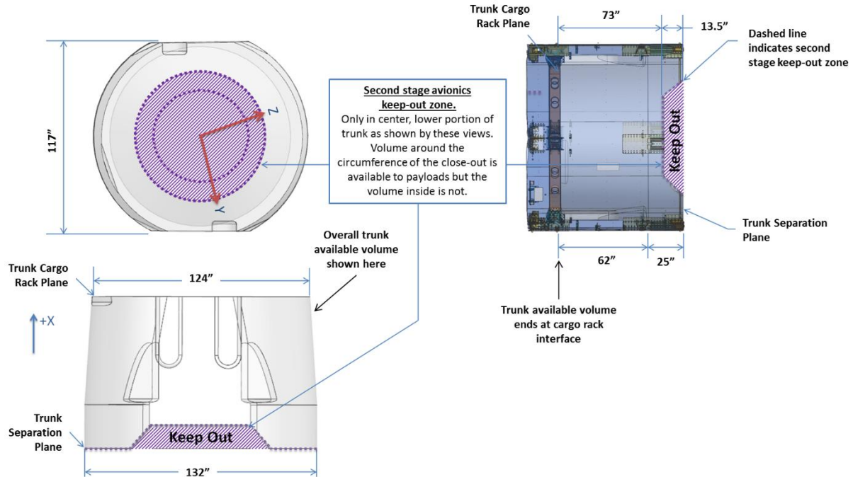
FIGURE 6.3.1-2 DRAGON MAJOR COMPONENTS
