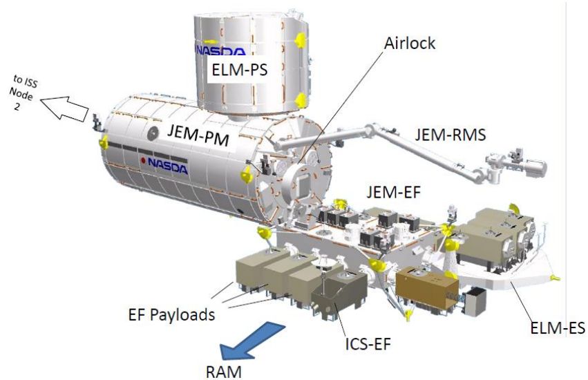
FIGURE 4.2-1 ILLUSTRATED JEM-EF OVERVIEW
