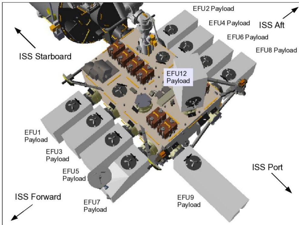
FIGURE 4.2.7-2 JEM-EF PAYLOAD VOLUME LOCATIONS AND ORIENTATIONS
