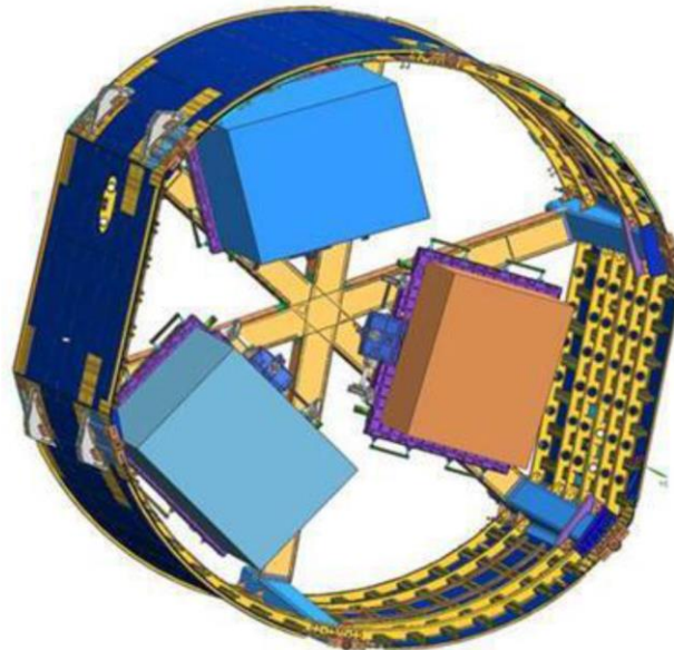
FIGURE 6.3.1-3 THREE FRAM-BASED UNPRESSURIZED CARGO ITEMS
