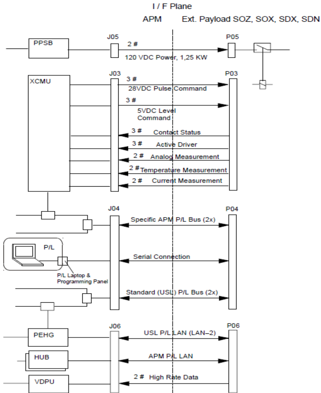
FIGURE 4.3.4-1 INTEGRATED EXTERNAL PAYLOAD SYSTEM INTERFACES
