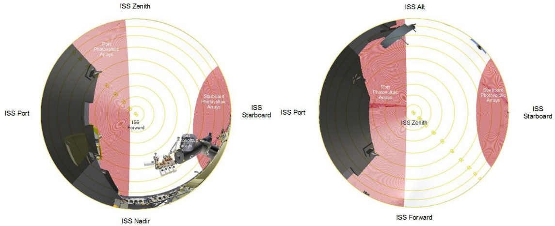
FIGURE 4.1.8-6 ELC-3 INBOARD EXPA PAYLOAD ACCOMMODATION FORWARD (RAM) AND ZENITH FOVS
