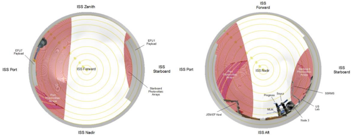
FIGURE 4.2.7-7 JEM-EF EFU3 PAYLOAD ACCOMMODATION FORWARD (RAM) AND NADIR)
