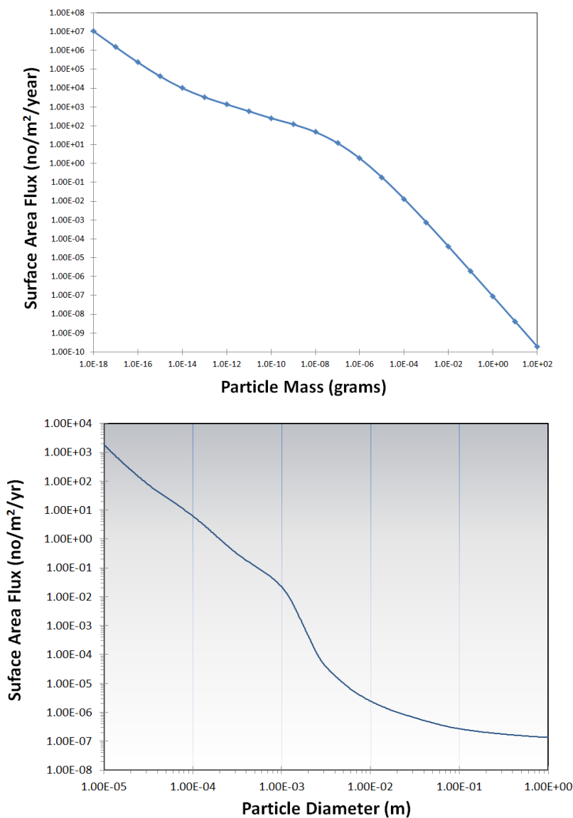
FIGURE 3.2.2-1 ARTIFICIAL SPACE DEBRIS ENVIRONMENT
