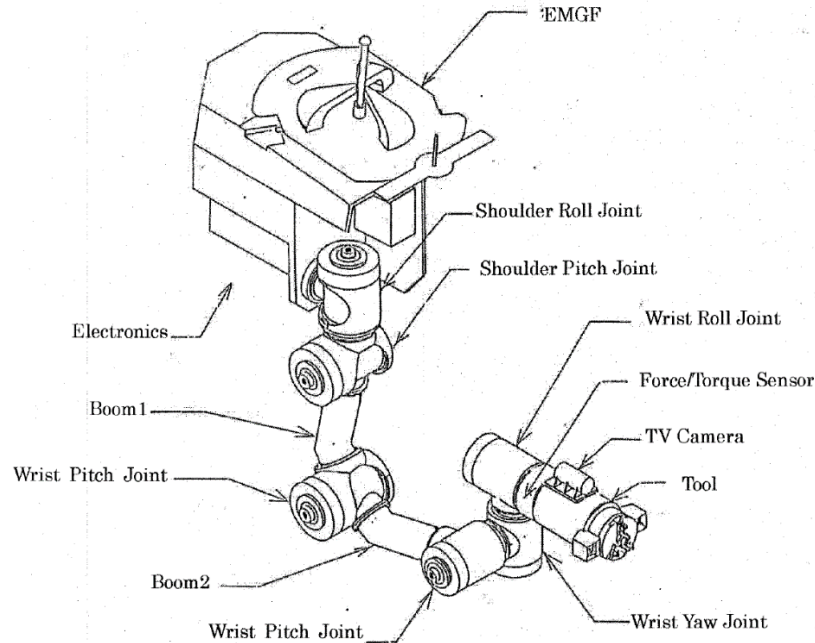
FIGURE 4.2.2-2 SFA CONFIGURATION
