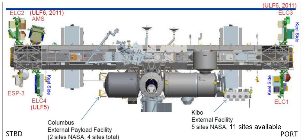
FIGURE 4.1.1-1 ELC LOCATIONS ON ISS
