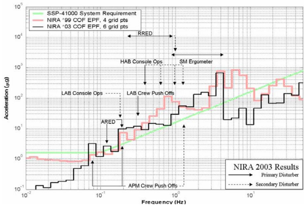
FIGURE 3.2.1-3 COLUMBUS MICROGRAVITY ENVIRONMENT
