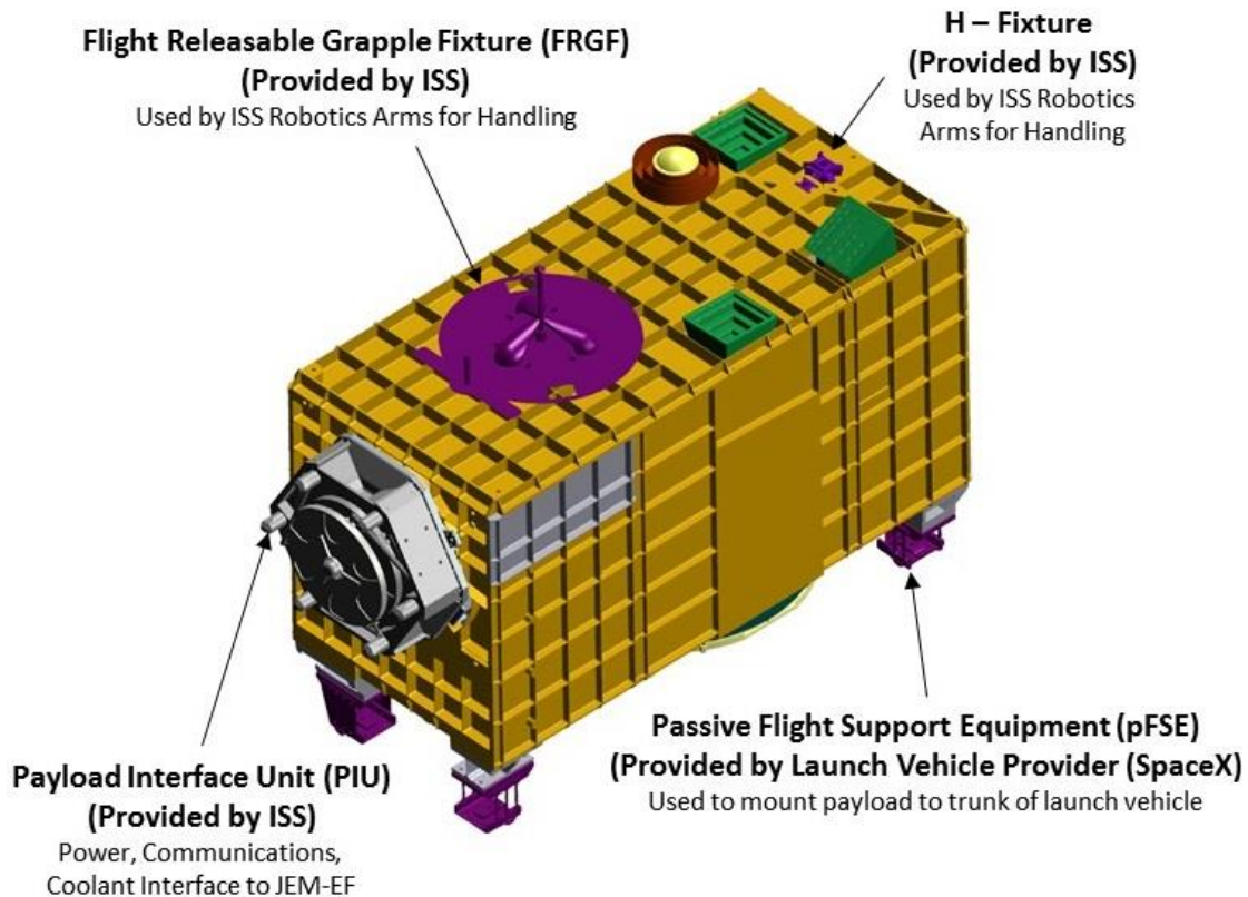
FIGURE 4.2.1-2 JEM-EF TYPICAL CONFIGURATION
