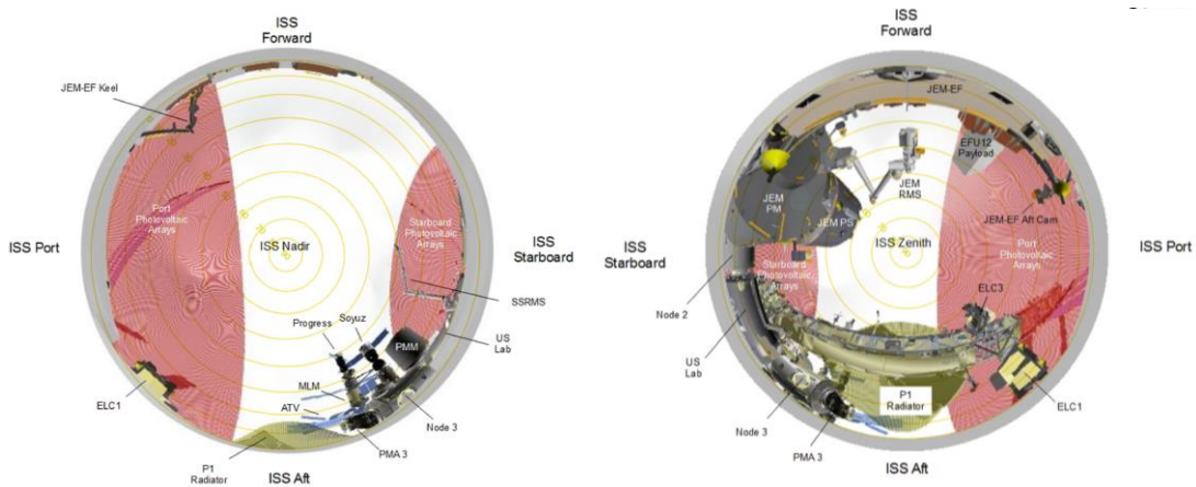
FIGURE 4.2.7-9 JEM-EF EFU4 PAYLOAD ACCOMMODATION NADIR AND ZENITH
