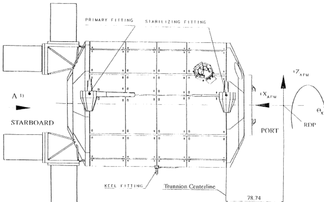
FIGURE 4.3-4 APM COORDINATE SYSTEM
