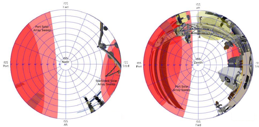
FIGURE 4.2.7-16 JEM-EF EFU10 PAYLOAD ACCOMMODATION NADIR AND ZENITH
