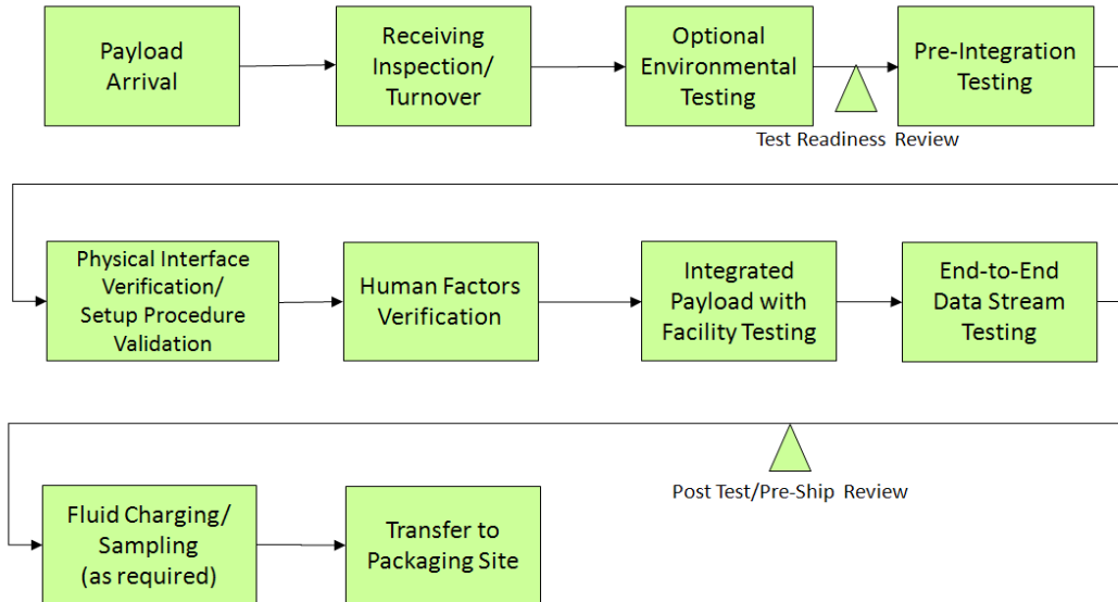
FIGURE 5.1.3-1 TESTING FLOW
