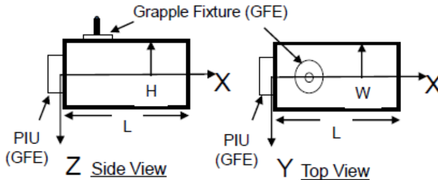
FIGURE 4.2.1-3 PAYLOAD INTERFACE UNIT
