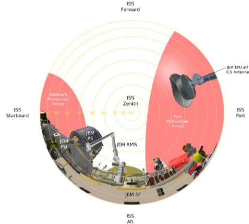
FIGURE 4.2.7-11 JEM-EF EFU5 PAYLOAD ACCOMMODATION FORWARD ZENITH
