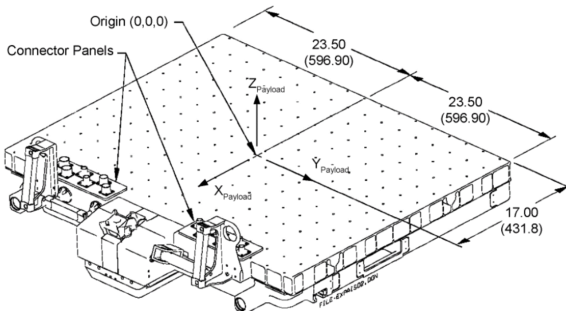
FIGURE 4.3.1-1 CEPA ISOMETRIC VIEW AND COORDINATE SYSTEM
