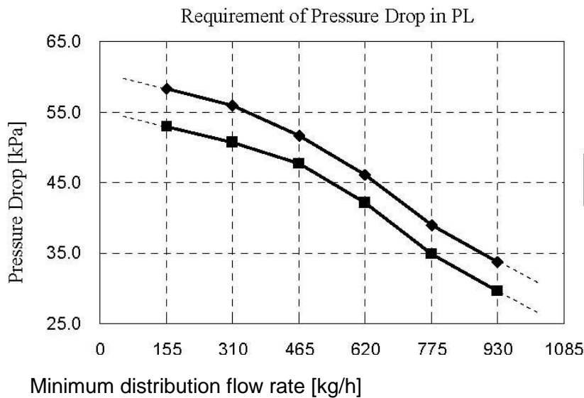
FIGURE 4.2.3.2-1 COOLANT PRESSURE DROP REQUIRED IN EXPERIMENT PAYLOAD
