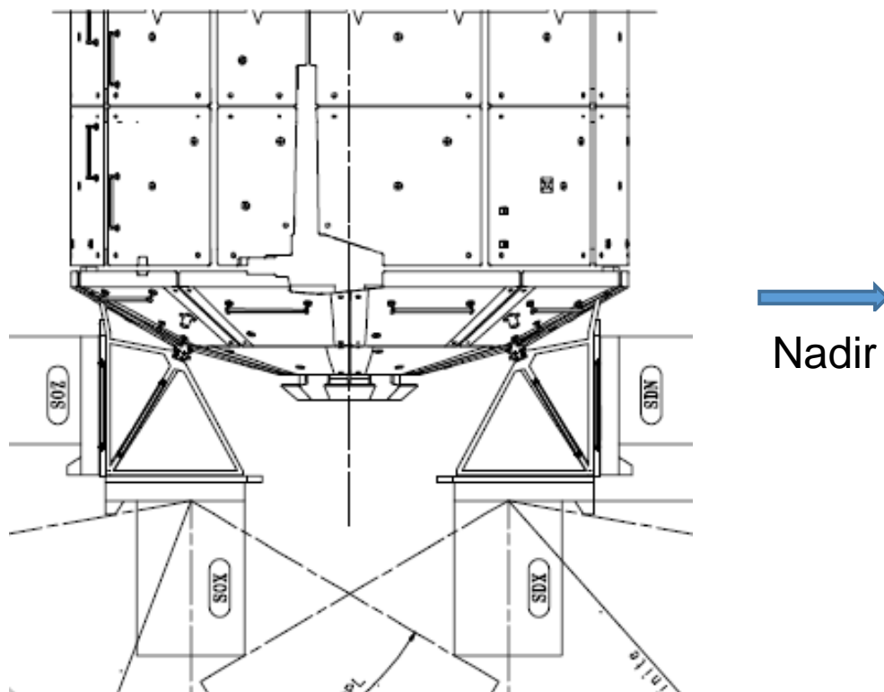
FIGURE 4.3-1 COLUMBUS EXTERNAL PAYLOAD SITES: SOZ, SOX, SDX, AND SDN
