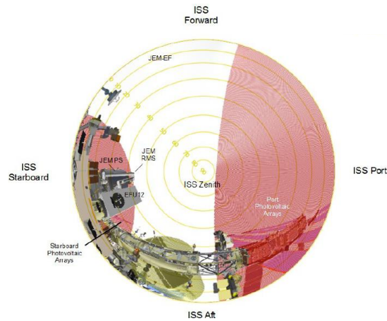
FIGURE 4.2.7-15 JEM-EF EFU9 PAYLOAD ACCOMMODATION ZENITH
