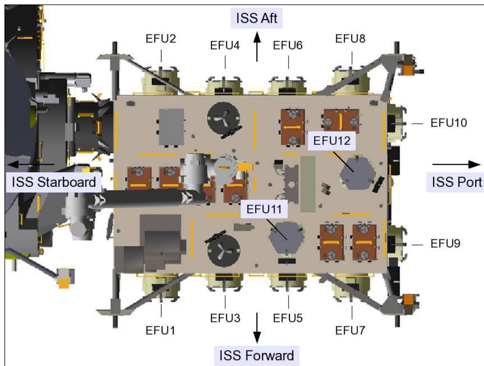
FIGURE 4.2.7-1 JEM-EF EFU LOCATIONS AND ORIENTATIONS
