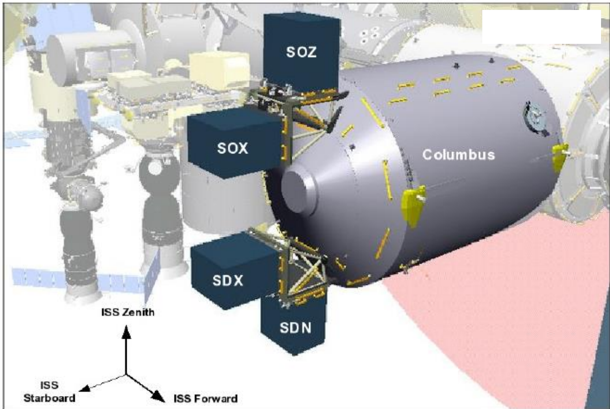
FIGURE 4.3.7-1 COLUMBUS-EPF OVERVIEW
