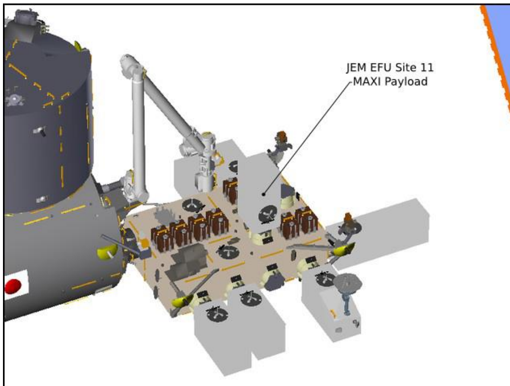
FIGURE 4.2.7-3 JEM-EF EFU PAYLOAD VOLUME LOCATIONS AND ORIENTATION
