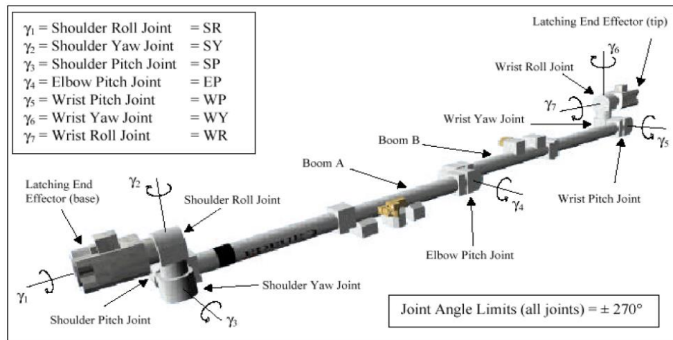
FIGURE 3.1.1-6 ISS SSRMS
