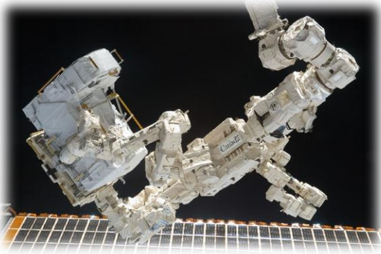
FIGURE 3.1.1-10 DEXTRE CARRIES PAYLOAD TO SITE
