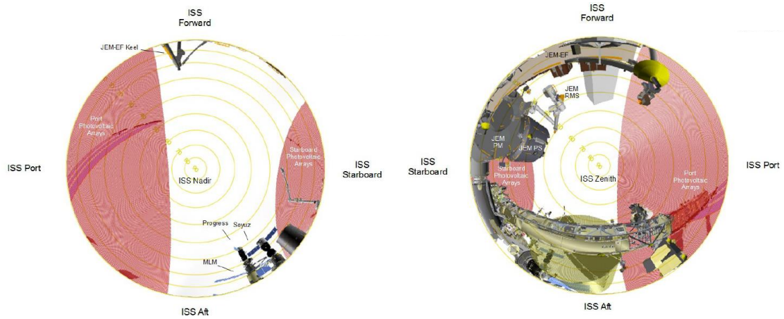
FIGURE 4.2.7-13 JEM-EF EFU8 PAYLOAD ACCOMMODATION NADIR AND ZENITH
