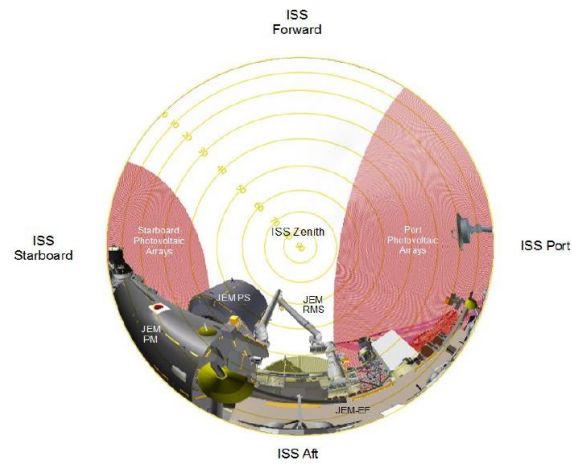
FIGURE 4.2.7-5 JEM-EF EFU1 PAYLOAD ACCOMMODATION ZENITH
