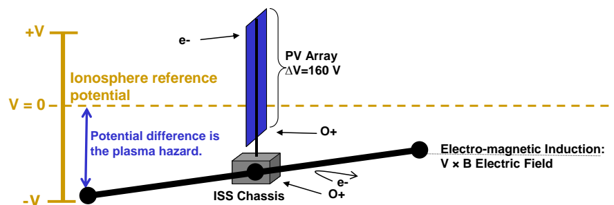
FIGURE 3.2.9-1 IONOSPHERE REFERENCE POTENTIAL-1
