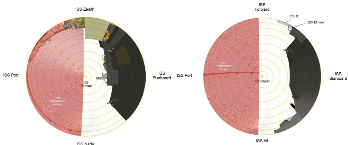
FIGURE 4.1.8-1 ELC-1 OUTBOARD EXPA PAYLOAD ACCOMMODATION FORWARD (RAM) AND NADIR
