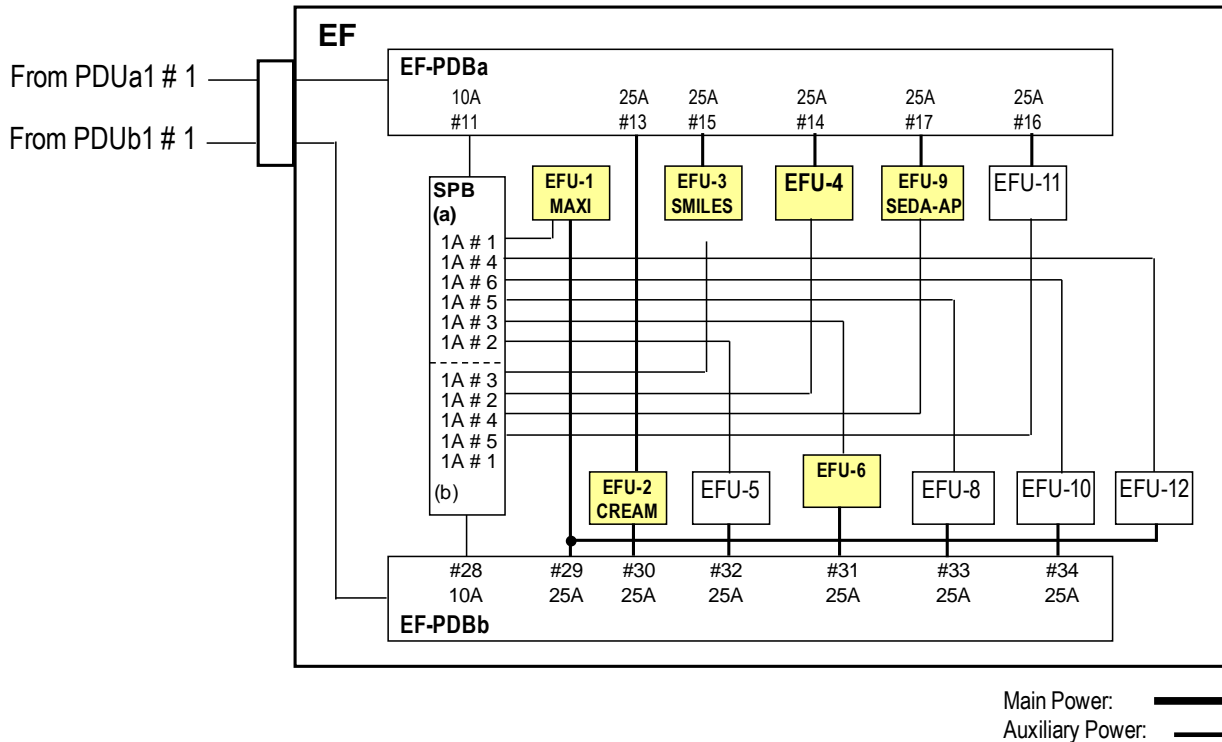
FIGURE 4.2.4-1 ELECTRIC POWER CONFIGURATION IN THE JPM
