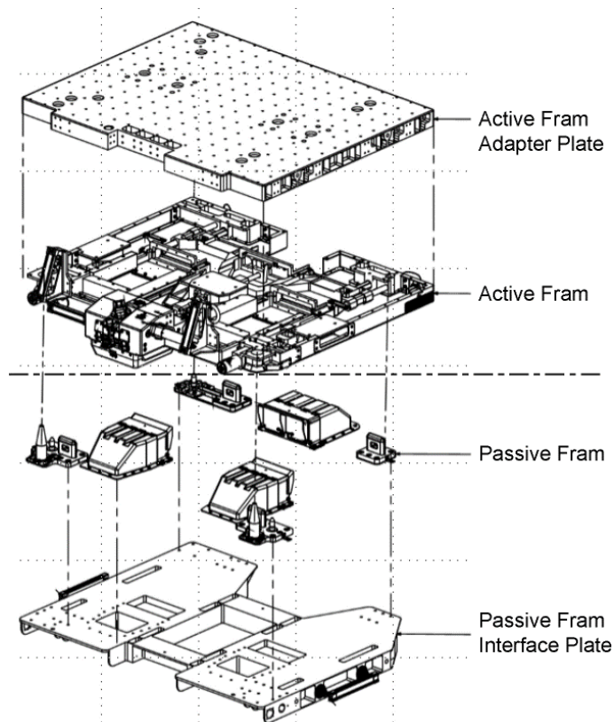
FIGURE 4.1.2-5 AFRAM AND PFRAM EXPENDED VIEW (NOTE: AFRAM ADAPTER PLATE AND THE AFRAM IS CONSIDERED A SINGLE UNIT)
