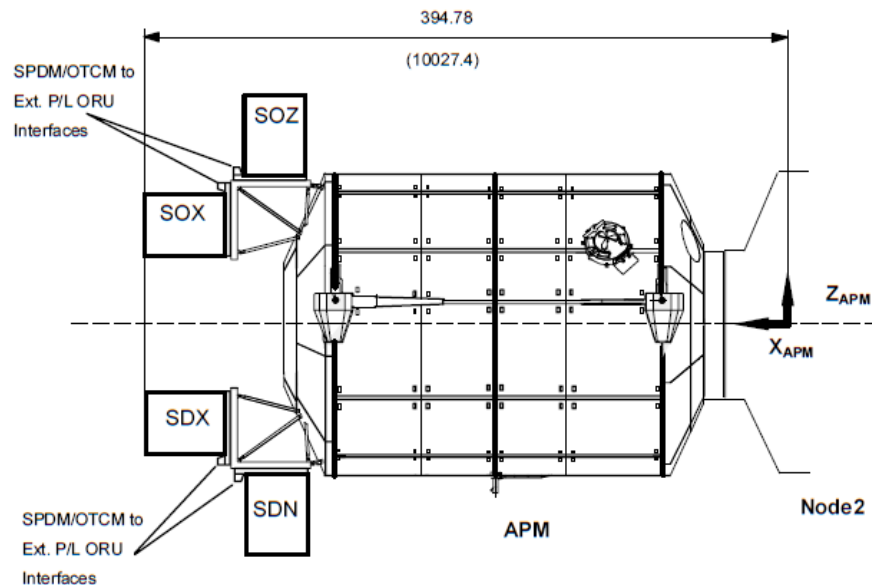
FIGURE 4.3-5 APM WITH EXTERNAL PAYLOADS AND OTCM LOCATIONS
