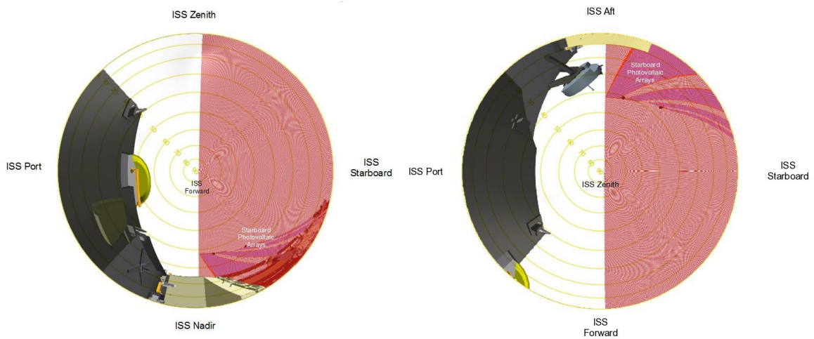
FIGURE 4.1.8-3 ELC-2 OUTBOARD EXPA PAYLOAD ACCOMMODATION FORWARD (RAM) AND ZENITH
