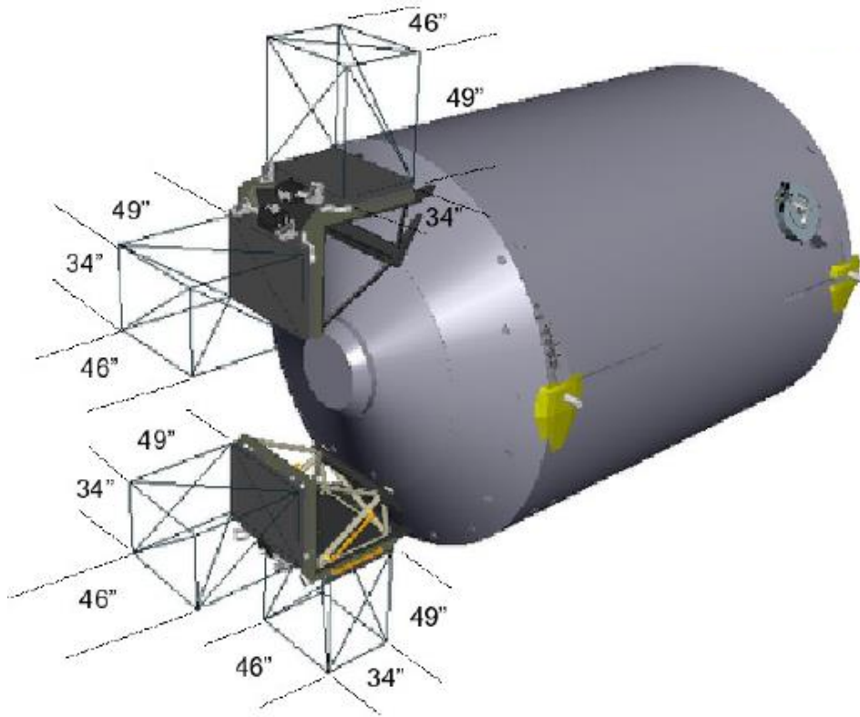
FIGURE 4.3.7-2 COLUMBUS-EPF PAYLOAD DIMENSIONS
