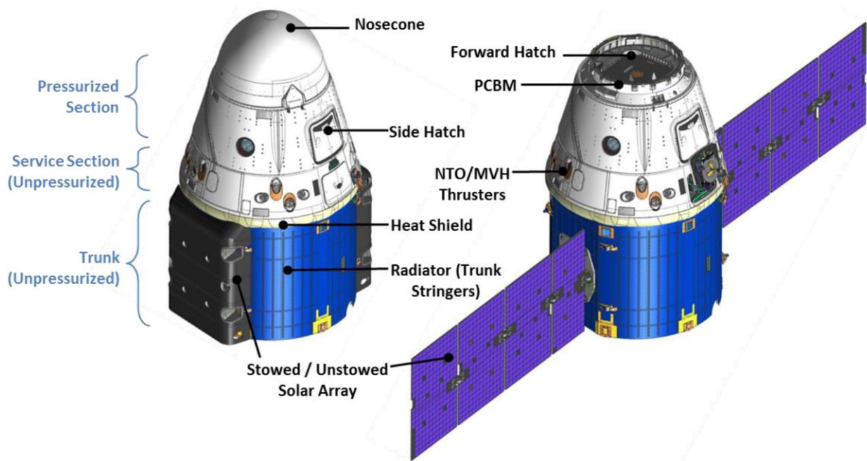
FIGURE 6.3.1-1 DRAGON COMPARTMENTS
