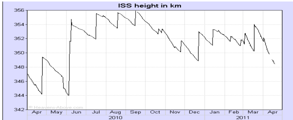
FIGURE 3.1.4-1A ISS ALTITUDE PROFILE
