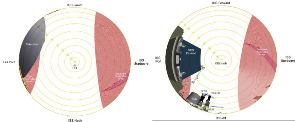
FIGURE 4.3.7-4 COLUMBUS SDX EXPA PAYLOAD ACCOMMODATION FORWARD (RAM) AND NADIR
