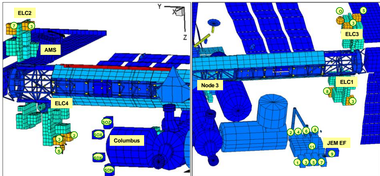
FIGURE 3.2.8-1 PAYLOAD MAPPING SITES (ELCS 1-4)
