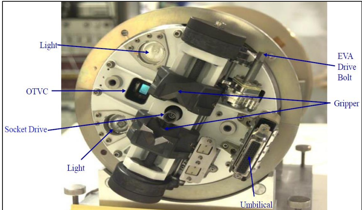
FIGURE 3.1.1-2 DEXTRE OTCM
