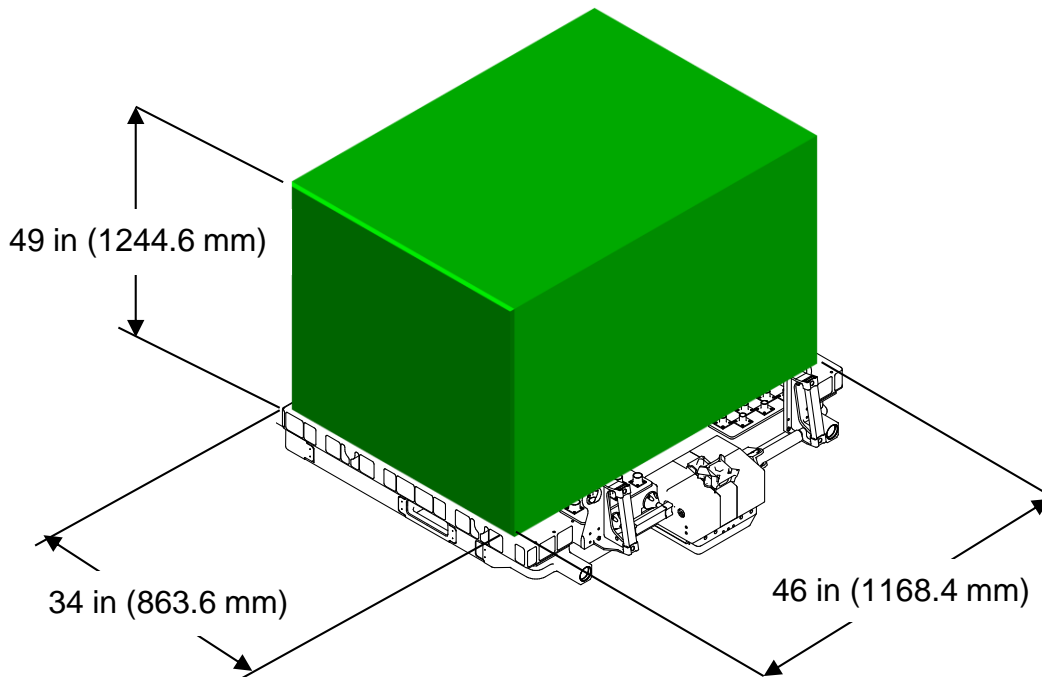
FIGURE 4.1.2-3 EXPA PAYLOAD ENVELOPE
