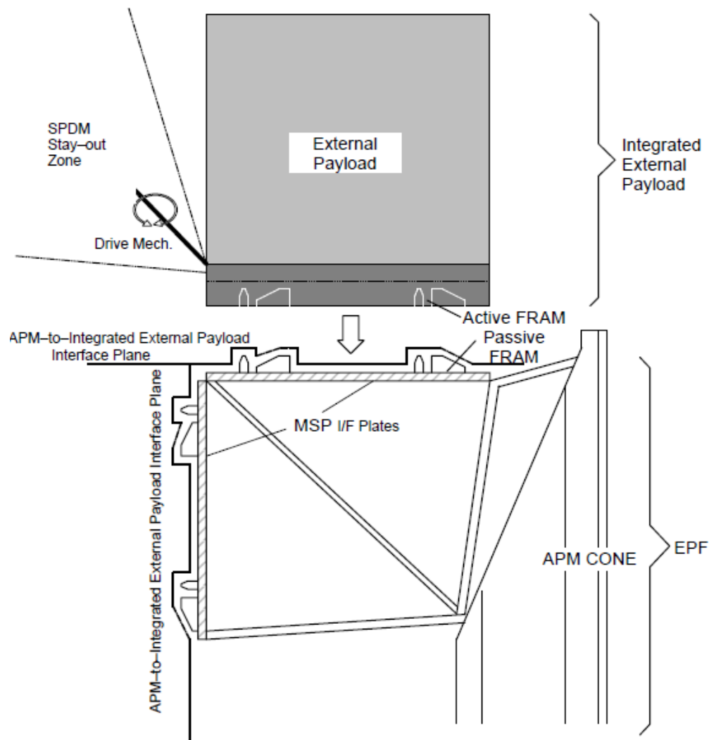
FIGURE 4.3.1-2 EXTERNAL PAYLOAD TO COLUMBUS ATTACHMENT
