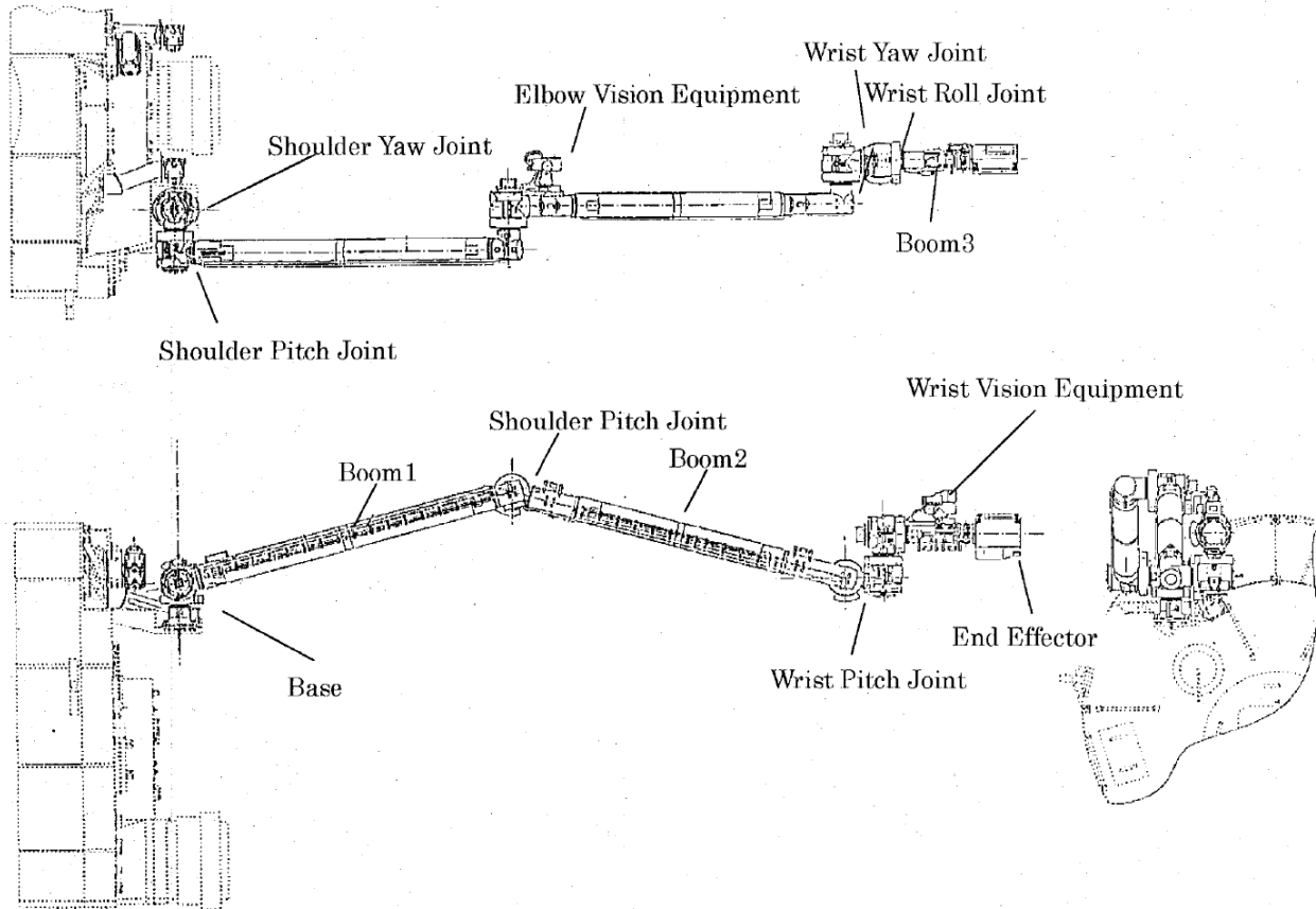
FIGURE 4.2.2-1 JEM-EF MA CONFIGURATION
