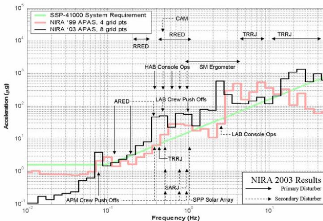
FIGURE 3.2.1-1 TYPICAL ELC MICROGRAVITY ENVIRONMENT
