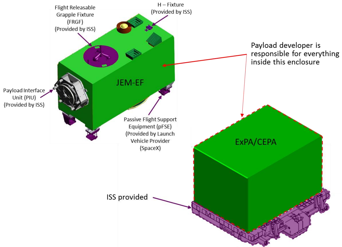
FIGURE 9.0-1 PD-PROVIDED HARDWARE INTERFACE PLANE
