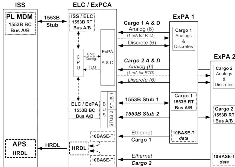
FIGURE 4.1.6-1 ISS TO EXPA C&DH BLOCK DIAGRAM
