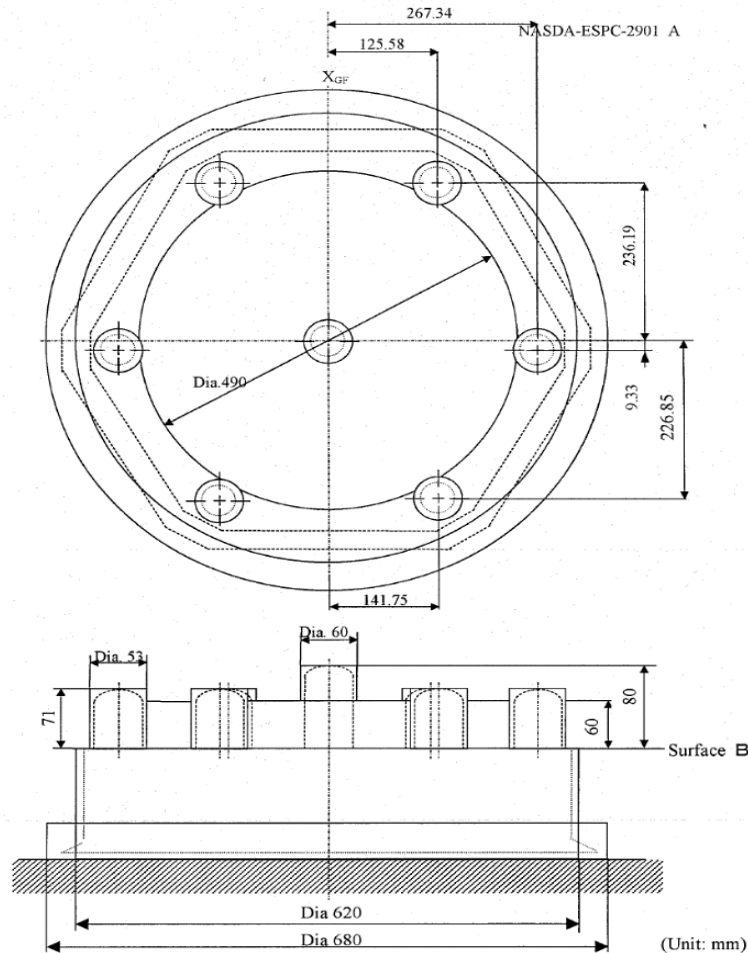
FIGURE 4.2.2-4 PIU DYNAMIC ENVELOPE
