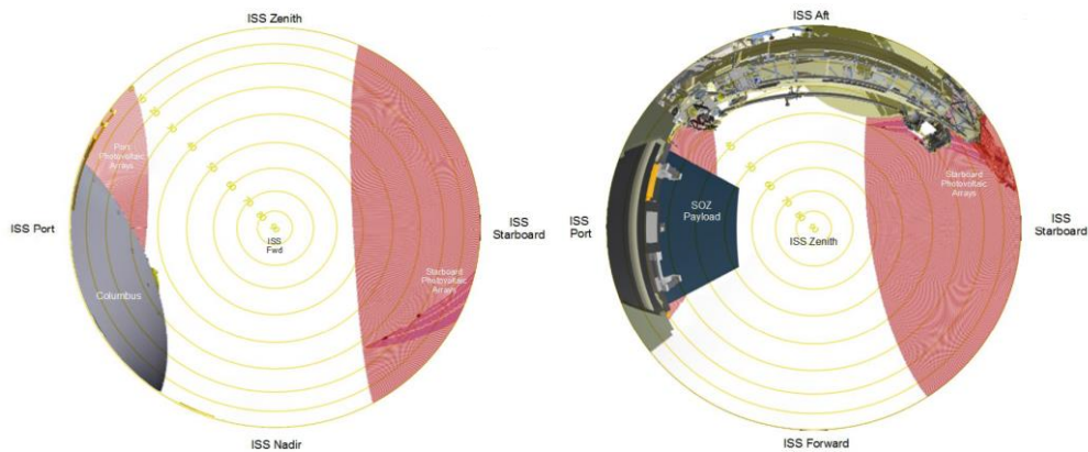
FIGURE 4.3.7-5 COLUMBUS SOX EXPA PAYLOAD ACCOMMODATION FORWARD (RAM) AND ZENITH
