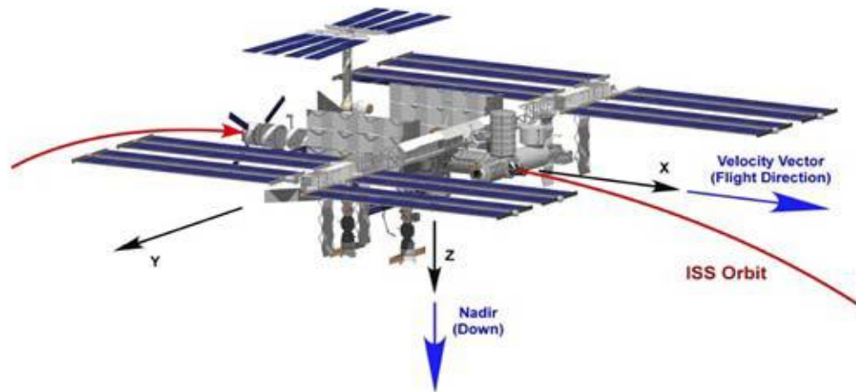
FIGURE 3.1.4-2 +XVV ORIENTATION OF ISS
