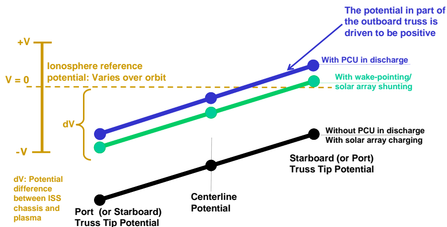
FIGURE 3.2.9-2 IONOSPHERE REFERENCE POTENTIAL-2
