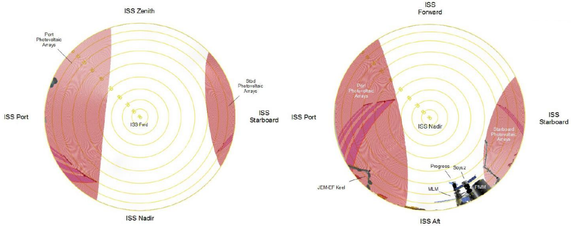
FIGURE 4.2.7-4 JEM-EF EFU1 PAYLOAD ACCOMMODATION FORWARD (RAM) AND NADIR)
