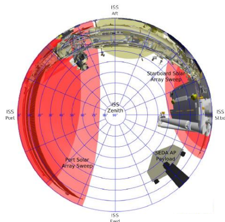
FIGURE 4.2.7-18 JEM-EF EFU12 PAYLOAD ACCOMMODATION ZENITH
