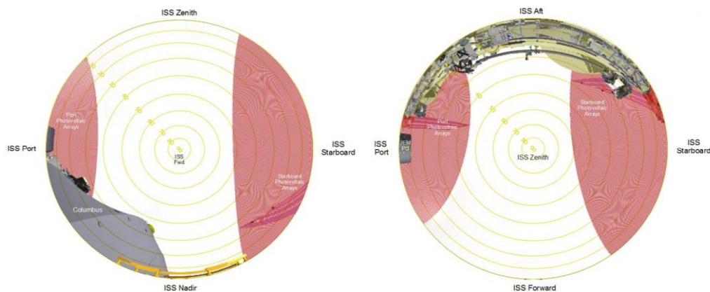
FIGURE 4.3.7-6 COLUMBUS SOZ EXPA PAYLOAD ACCOMMODATION FORWARD (RAM) AND ZENITH
