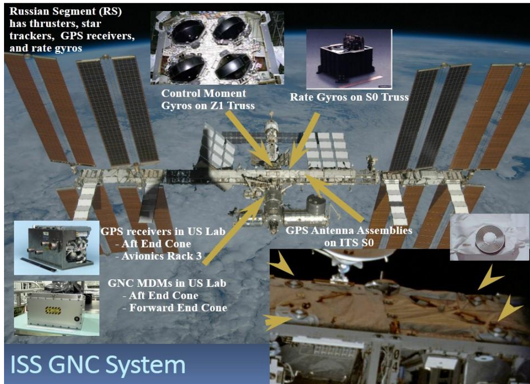
FIGURE 3.1.5-1 ISS GN&C SYSTEM
