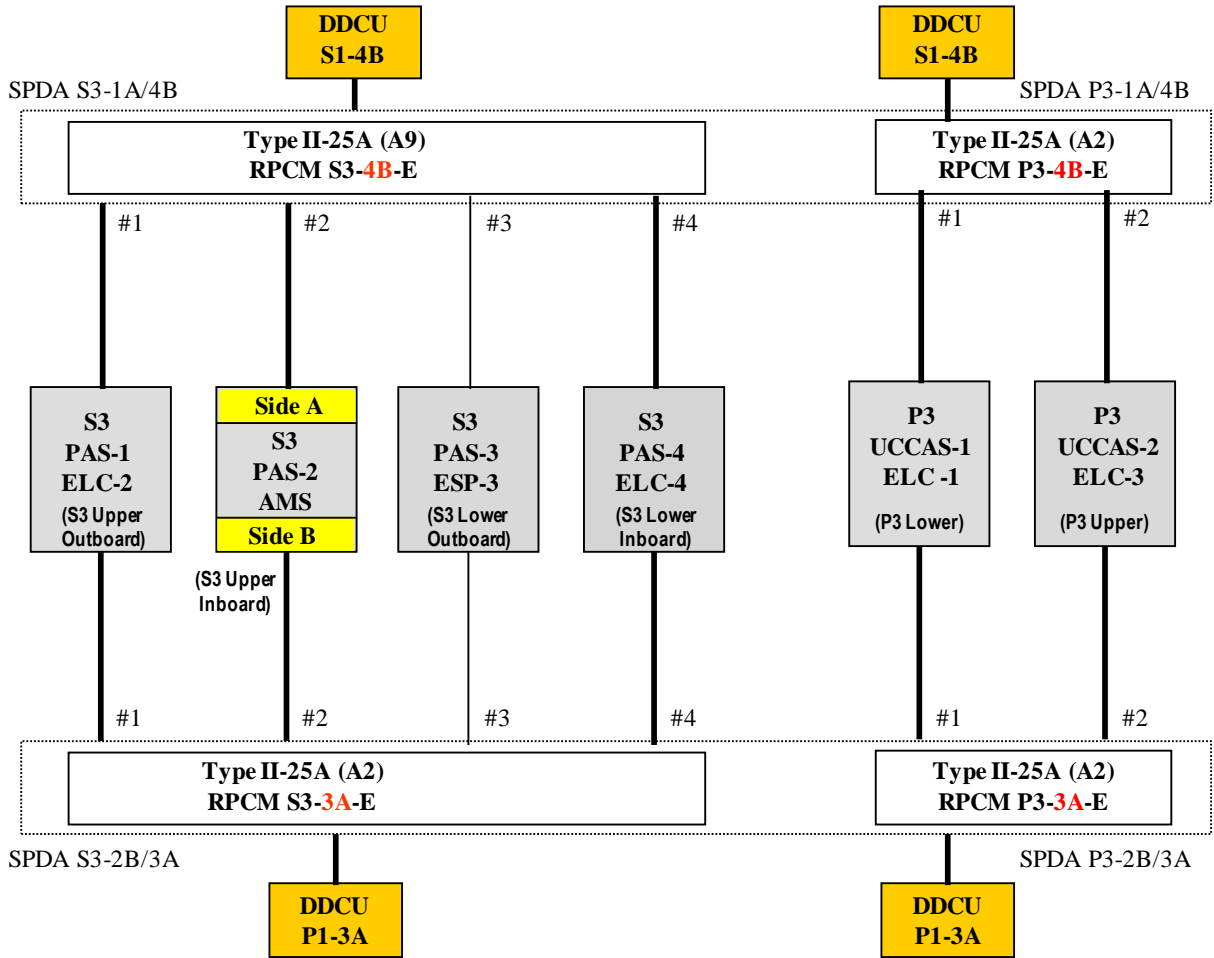
FIGURE 4.1.5-1 ISS ITA INTERFACES
