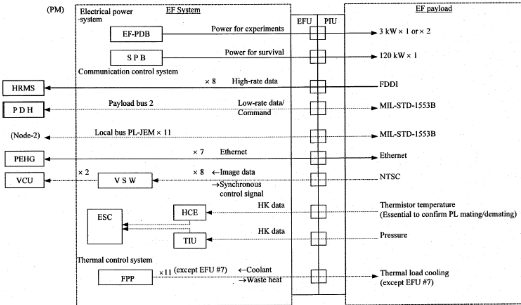
FIGURE 4.2.5-1 POWER AND DATA CONNECTIONS
