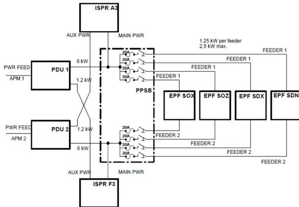
FIGURE 4.3.4-3 EXTERNAL PAYLOAD POWER DISTRIBUTION
