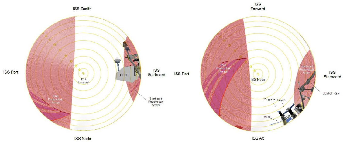
FIGURE 4.2.7-14 JEM-EF EFU9 PAYLOAD ACCOMMODATION FORWARD (RAM) AND NADIR)
