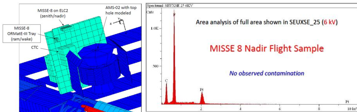
FIGURE 3.2.8-2 MISSE 8 CONFIGURATION ON ELC2 AND SAMPLE SURFACE ANALYSIS RESULTS
