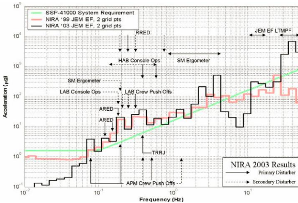
FIGURE 3.2.1-2 TYPICAL MICROGRAVITY ENVIRONMENT FOR JEM-EF
