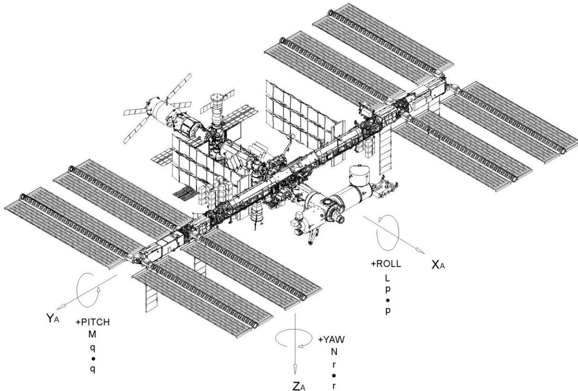
FIGURE 3.1.5-3 ISS DYNAMIC REFERENCES
