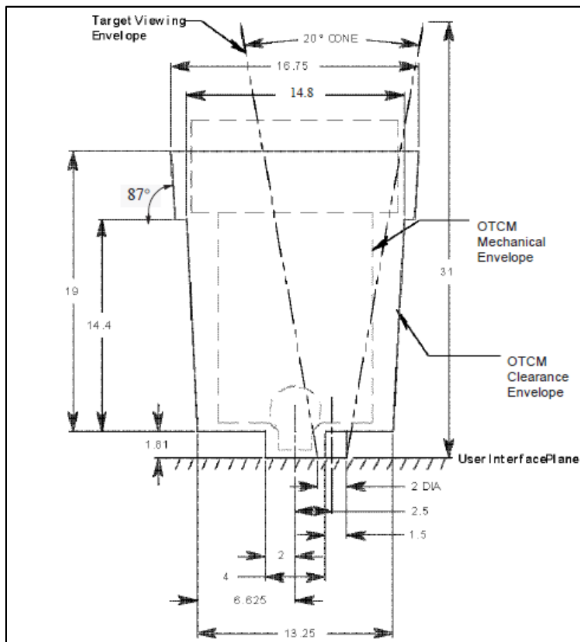
FIGURE 3.1.1-3 DEXTRE INTERFACES
