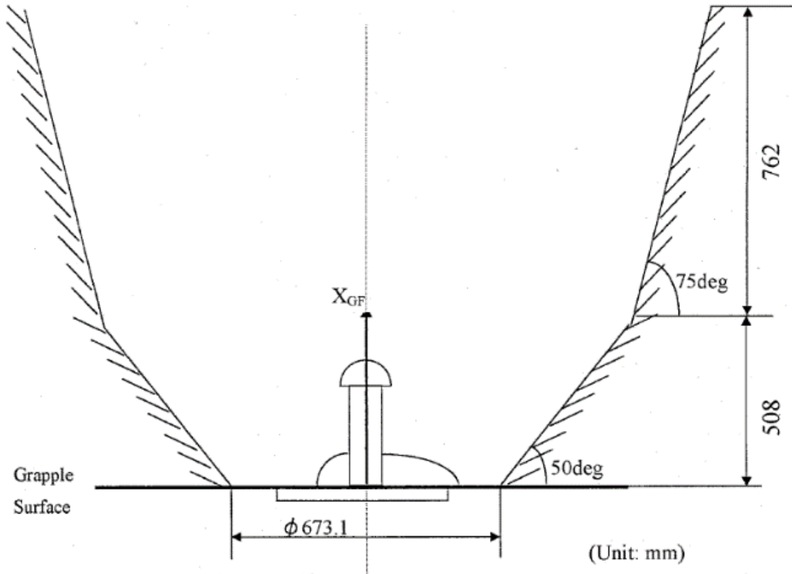
FIGURE 4.2.2-3 ILLUSTRATION OF CLEARANCE FOR THE MA AND PAYLOAD GRAPPLING OPERATION
