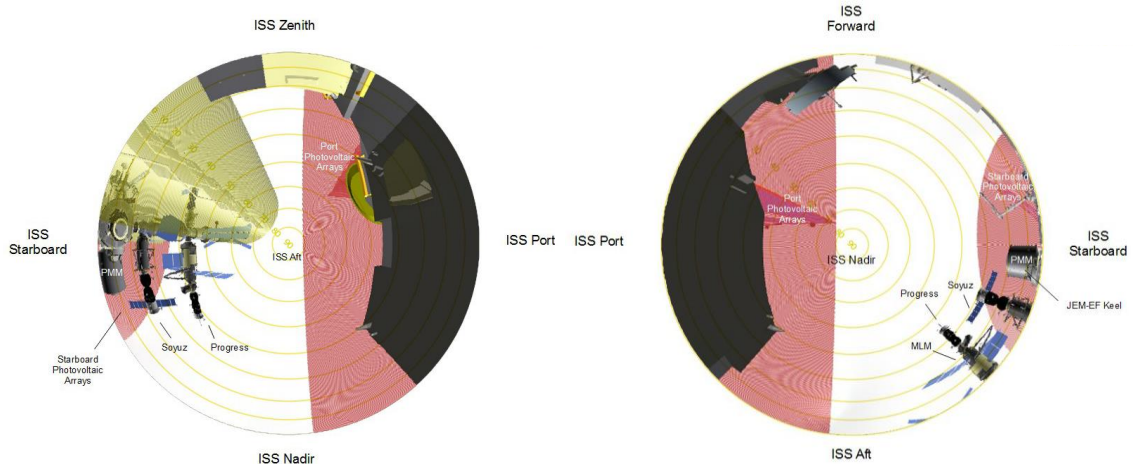
FIGURE 4.1.8-2 ELC-1 INBOARD EXPA PAYLOAD ACCOMMODATION AFT (WAKE) AND NADIR
