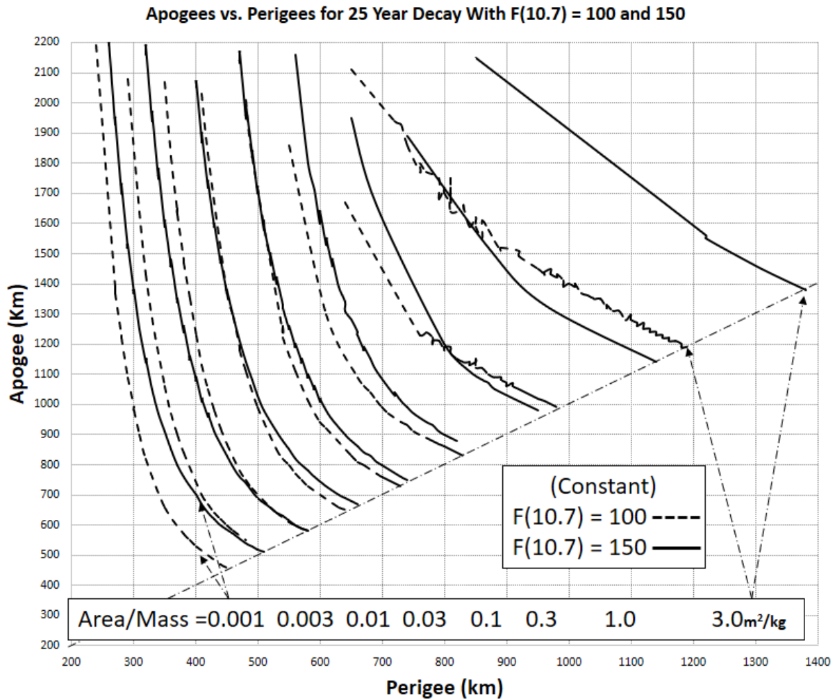
Figure 4.3-1. Apogee vs. Perigees for 25 Year Decay With F(10.7) = 100 and 150
